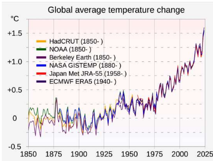
Figure 0.3: Correlation of measured global average temperature, from several different scientific organizations
